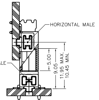
Mating Application - Daughter Card to Motherboard
