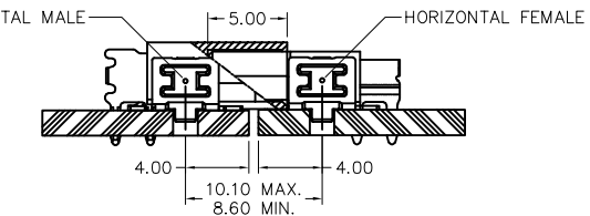
Mating Application - Extender Card
