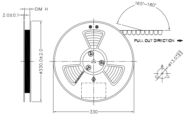
PULL OUT DIRECTION → CARRIER DIMENSION - 2P to 3P
