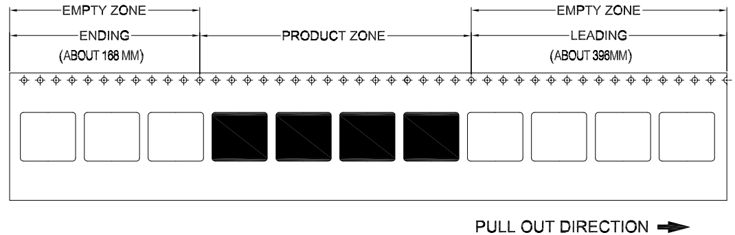
PULL OUT DIRECTION → CARRIER DIMENSION - 4P to 12P
