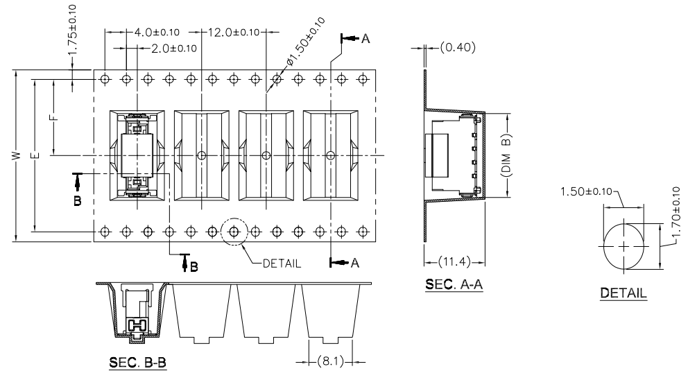
PULL OUT DIRECTION → CARRIER DIMENSION - 4P to 12P
