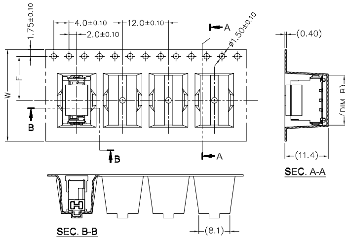
PULL OUT DIRECTION → CARRIER DIMENSION - 2P to 3P
