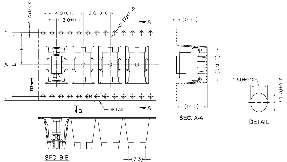
SEC. B-B
