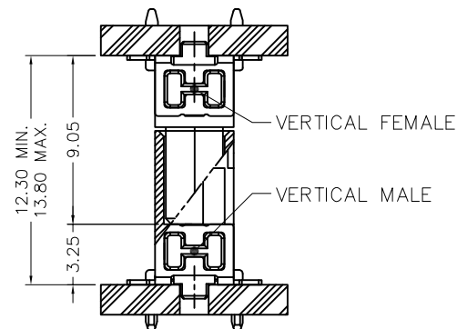
Mating Application— Board to Board Stacking
