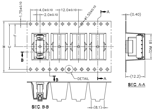
SEC. A-A SEC. B-B PULL OUT DIRECTION ➡ CARRIER DIMENSION - 4P to 12P
