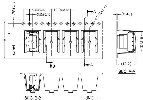
SEC. A-A SEC. B-B PULL OUT DIRECTION ➡ CARRIER DIMENSION - 2P to 3P
