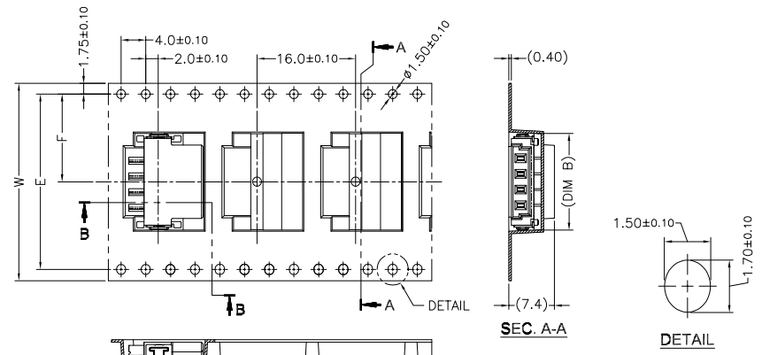
PULL OUT DIRECTION → CARRIER DIMENSION - 4P to 12P
