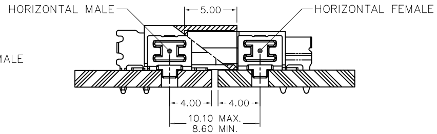
Mating Application— Extender Card
