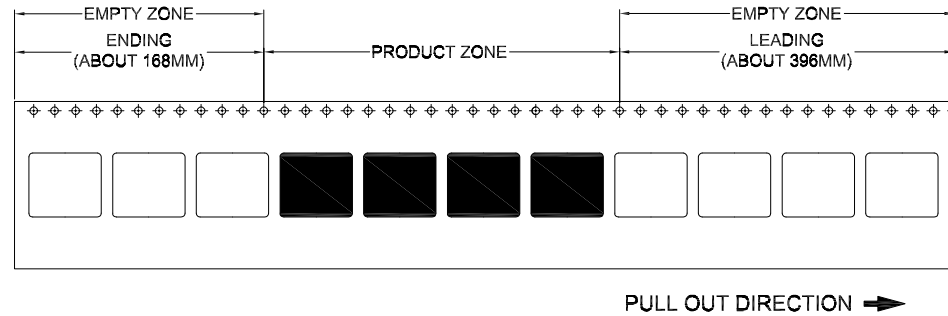
PULL OUT DIRECTION → CARRIER DIMENSION - 4P to 12P
