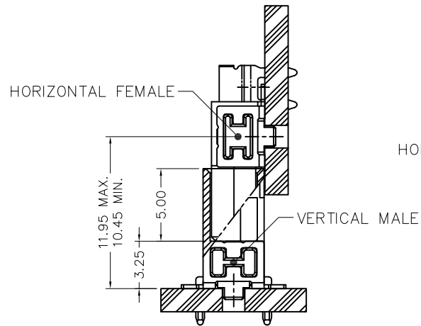
Mating Application— Daughter Card to Motherboard
