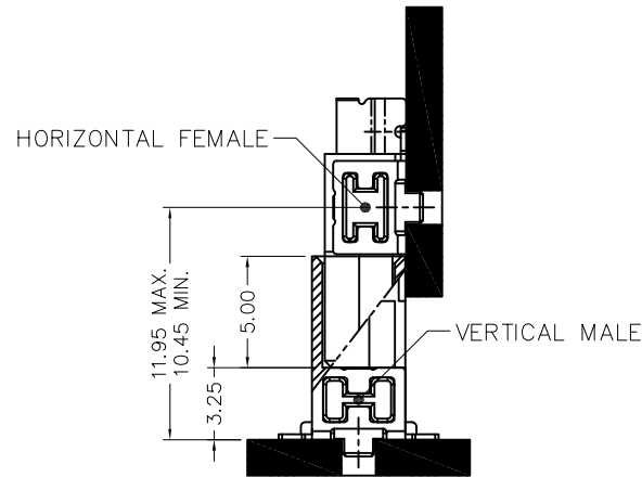
Mating Application - Daughter Card to Motherboard
