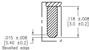
PEG DETAIL B
