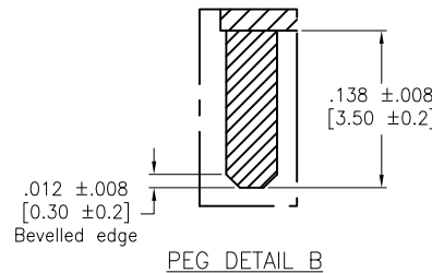
PEG DETAIL B
