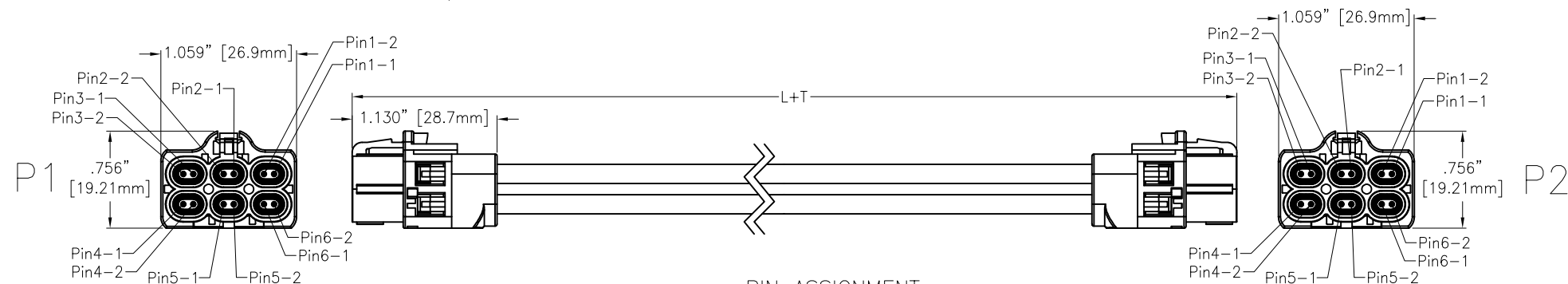
PIN ASSIGNMENT
