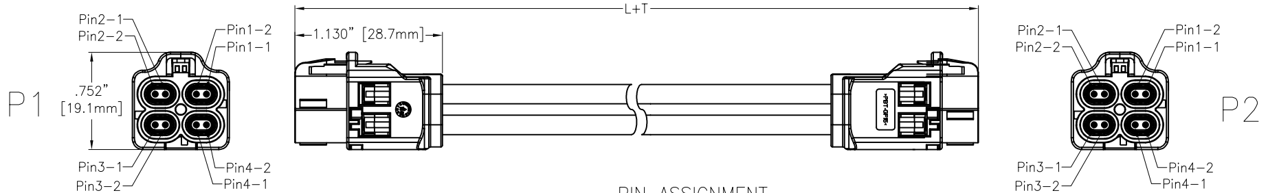
PIN ASSIGNMENT
