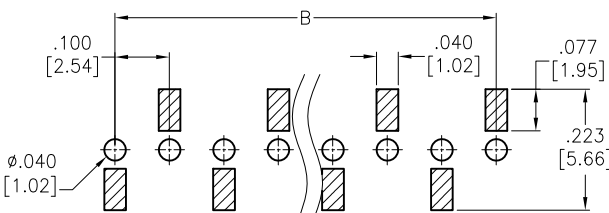
RSVL-1F-XX-G-SMT-B-PP-TR
