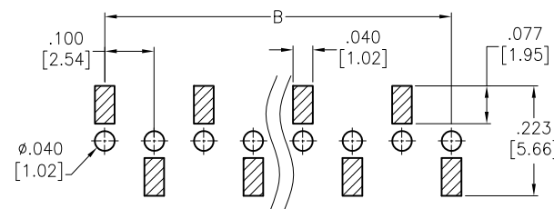
RSVL-1F-XX-G-SMT-A-PP-TR
