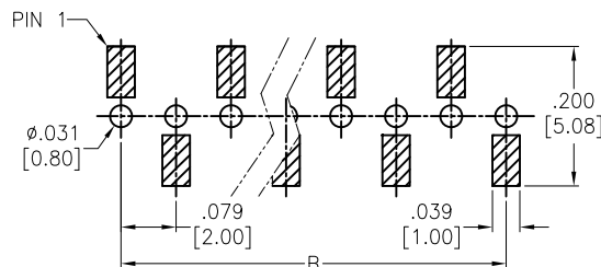
RECOMMENDED PCB LAYOUT Bottom Entry Optional
