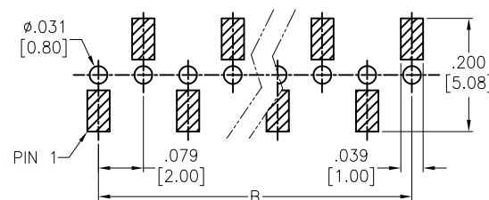
RECOMMENDED PCB LAYOUT Bottom Entry Optional
