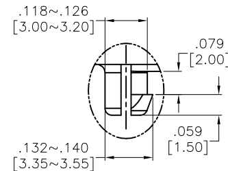
DETAIL Z
