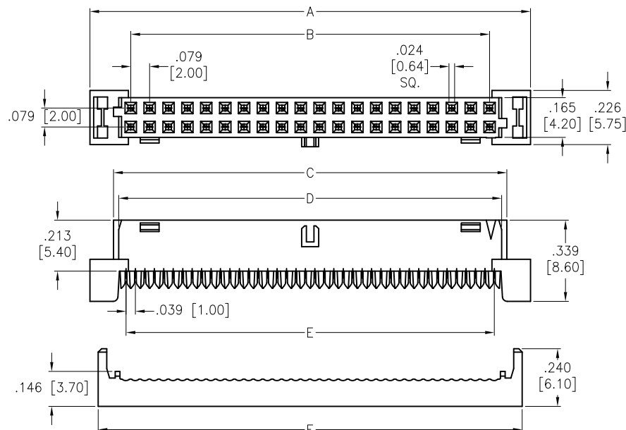
POLARIZATION AND RAMP LOCKING (APPLICABLE FOR 14 TO 50 CKT)
