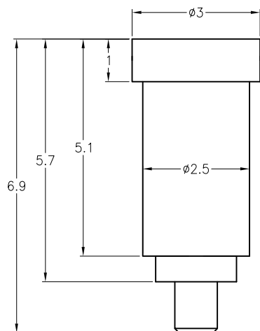
WITH CAP
