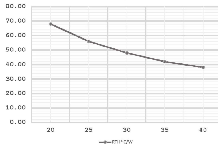
length (mm) vs R_{TH} ( ^{\circ}\text{C}/\text{Watt} )
