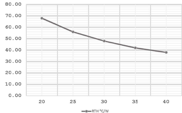
length (mm) vs R_{TH} ( ^{\circ}\text{C}/\text{Watt} )
