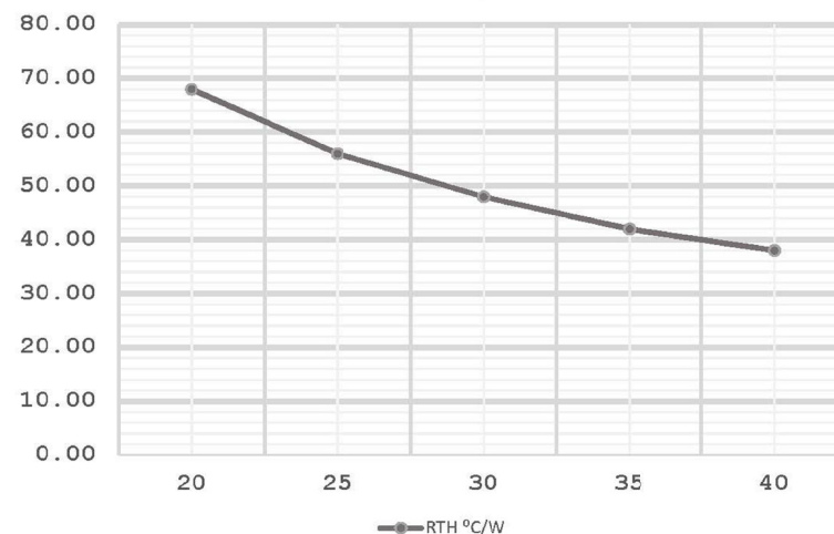
length (mm) vs R_{TH} ( ^{\circ}\text{C}/\text{Watt} )
