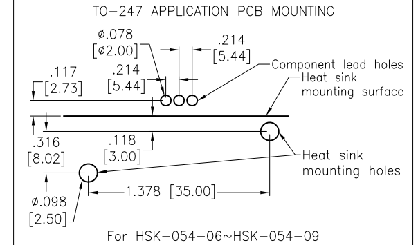
TO-220/TO-247 TRANSISTOR MOUNTING ORIENTATION
