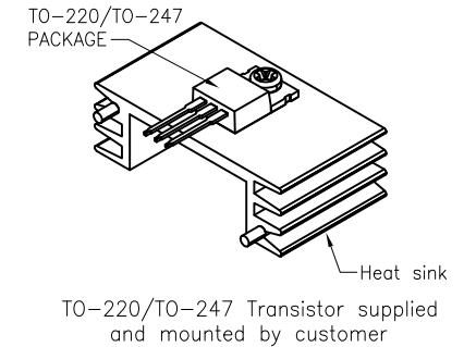
TO-220/TO-247 TRANSISTOR MOUNTING ORIENTATION
