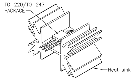
TO-220/TO-247 TRANSISTOR MOUNTING ORIENTATION
