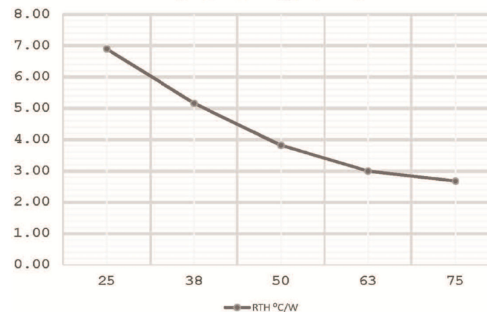
length (mm) vs R_{TH} ( ^{\circ}C/Watt )
