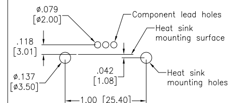
APPLICATION PCB MOUNTING
