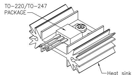
TO-220/TO-247 TRANSISTOR MOUNTING ORIENTATION
