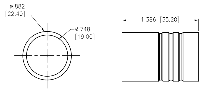
Seal Ring For 4/0AWG (350A)&95mm 2 (300A) (Packaged separately in poly bag)
