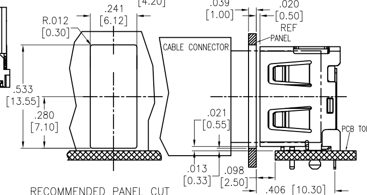
RECOMMENDED PANEL CUT
