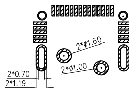
RECOMMENDED STENCIL LAYOUT
