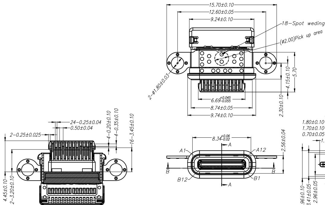
Section B-B
