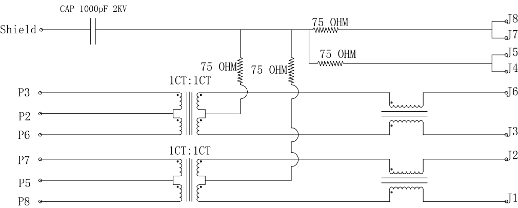
Circuit Schematic:
