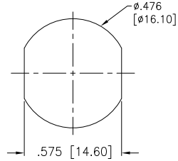
Panel Cut-Out (Front Panel Mounting)
