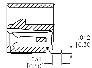
SECTION X-X
