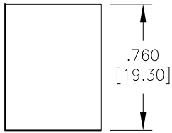
RECOMMENDED PANEL CUTOUT FOR SINGLE WALL PLATE AND BACK PANEL FOR DOUBLE WALL PLATE
