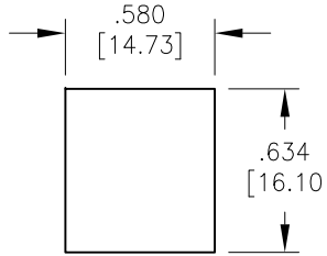
RECOMMENDED FRONT PANEL CUTOUT FOR DOUBLE WALL PLATE
