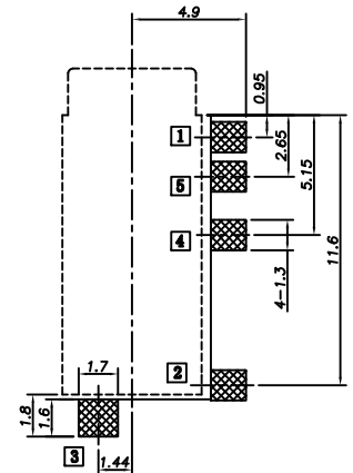
RECOMMENDED PCB LAYOUT (COPPER SIDE)
